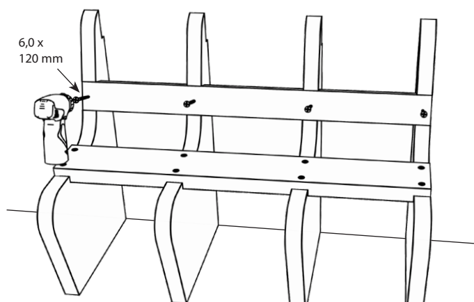
6) Glue on strut C2. Align supporting panels A the same distances apart and bolt on.
