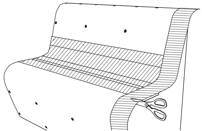
24) Tape over cover B2, all butt joints and visible edges with JACKOBOARD® self-adhesive glass fibre tape.
