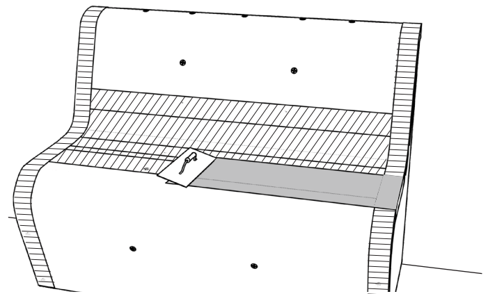
26) Apply tile adhesive over the glass fibre tape.
