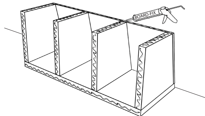
9) The bench must be glued to the wall and the floor. To do this, apply BOARD-FIX® to the front surfaces of the back and underside.
