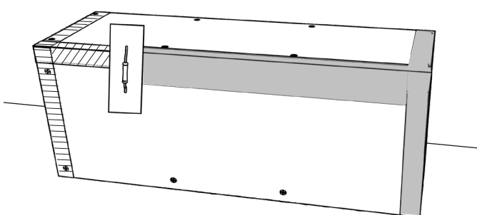
12) Apply tile adhesive over the glass fibre tape. The bench is now finished and can be tiled.
