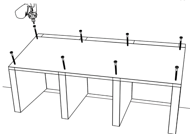
8) Glue on cover B2 and bolt in place.
