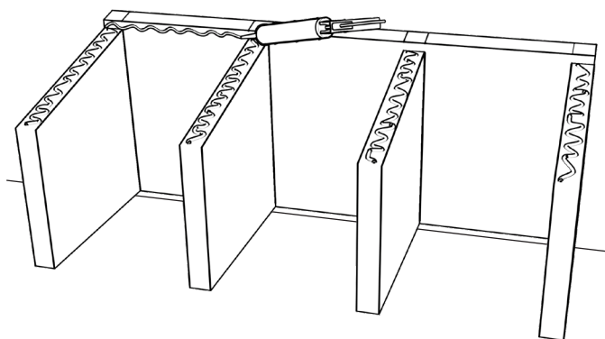
7) Apply BOARD-FIX® to supporting panels A and to the underside of cover B1.
